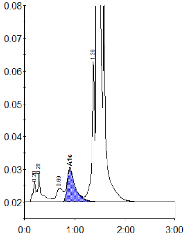
Peak table - ID: 10564318
